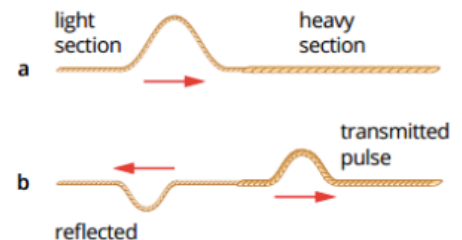
FIGURE 10.3.4 (a) A wave pulse travels along a light rope towards a heavier rope. (b) On reaching a change in density the wave pulse will be partly reflected and partly transmitted. This is analogous to a change in medium.
