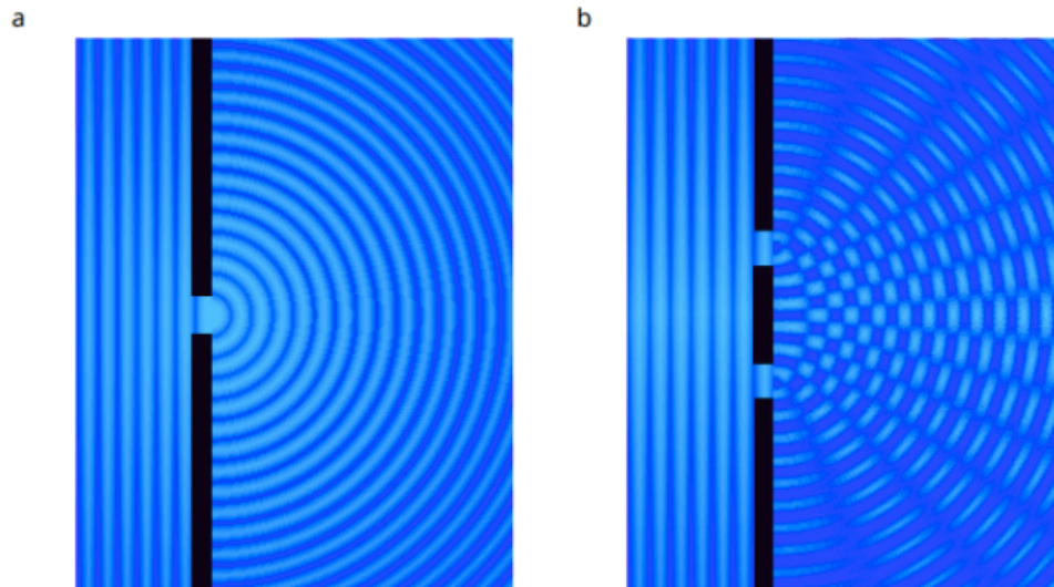
FIGURE 10.3.15 (a) A plane wave undergoes diffraction after passing through an aperture. (b) Interference effects occur due to diffraction from both of the slits.
