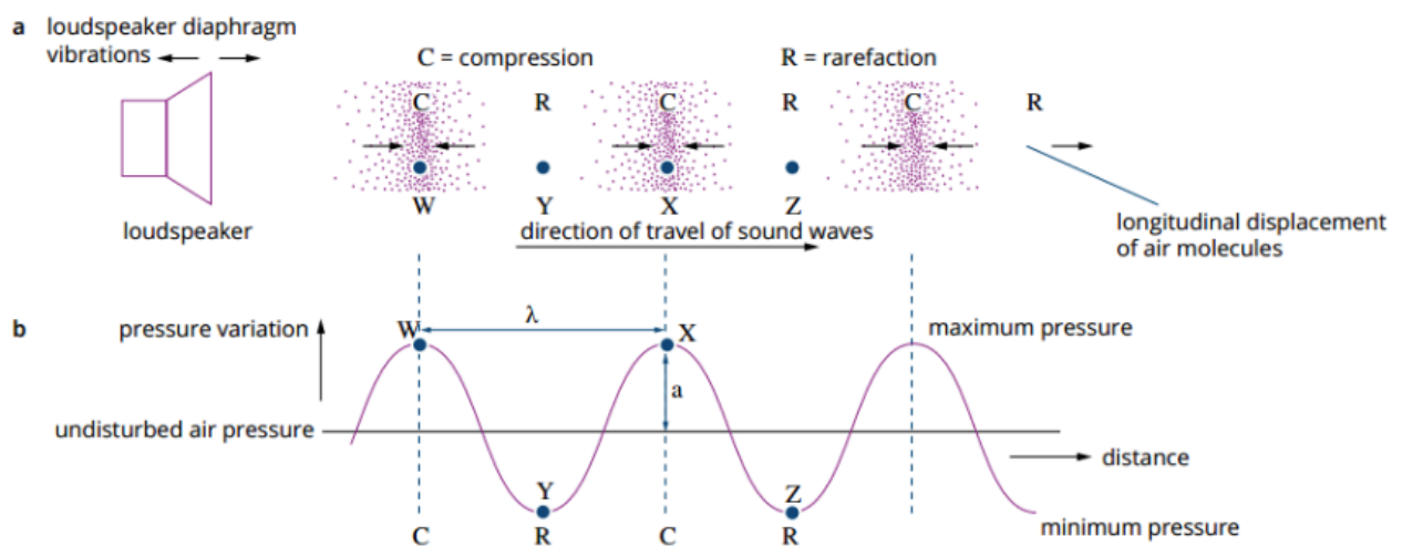
FIGURE 10.1.7 A longitudinal wave compared to a transverse wave. The compressions in a longitudinal wave are equivalent to a crest or peak in a transverse wave, and the rarefactions are equivalent to a trough.
